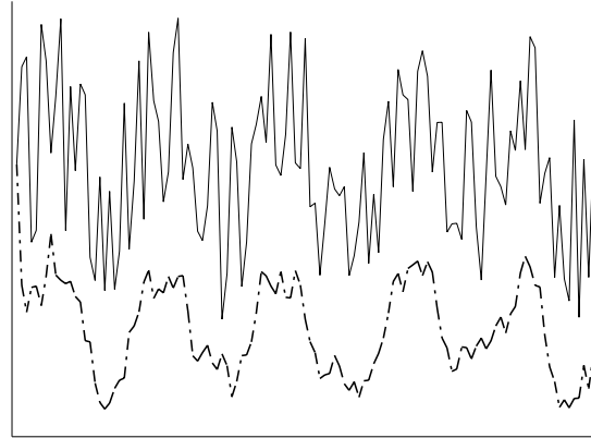
Figure A1. Noisy data smoothed by convolution.
